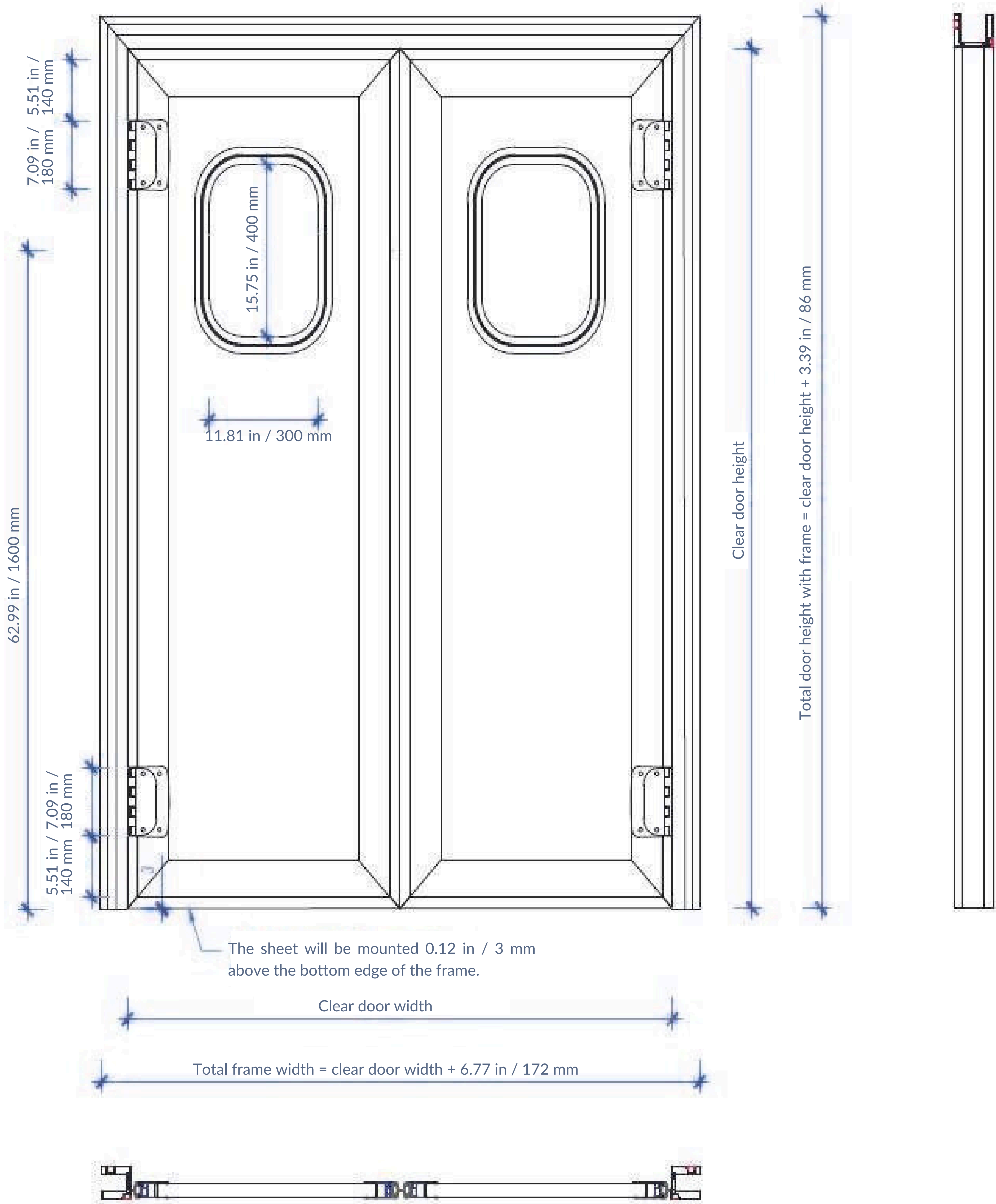
2-leaves swing refrigerator door
